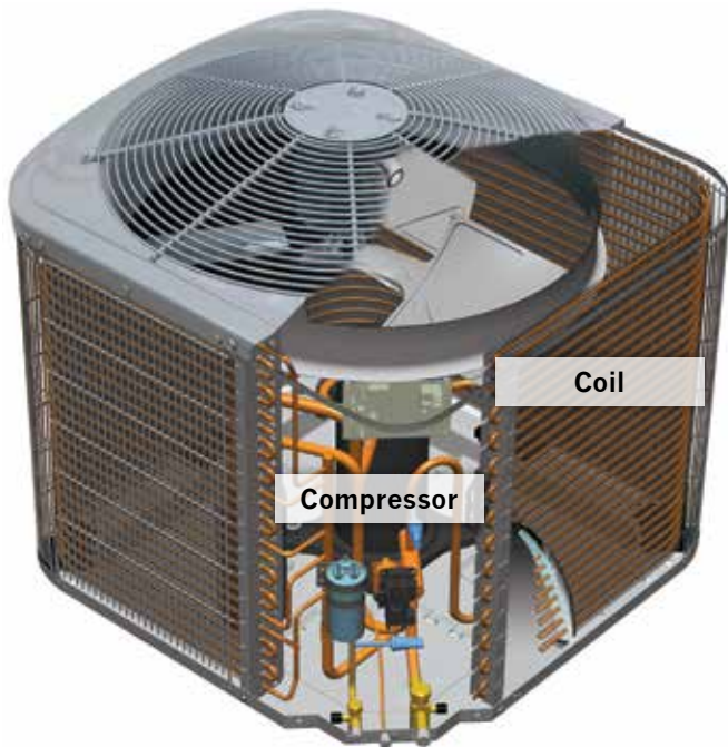
Comfort™ 15 Heat Pump Shown
